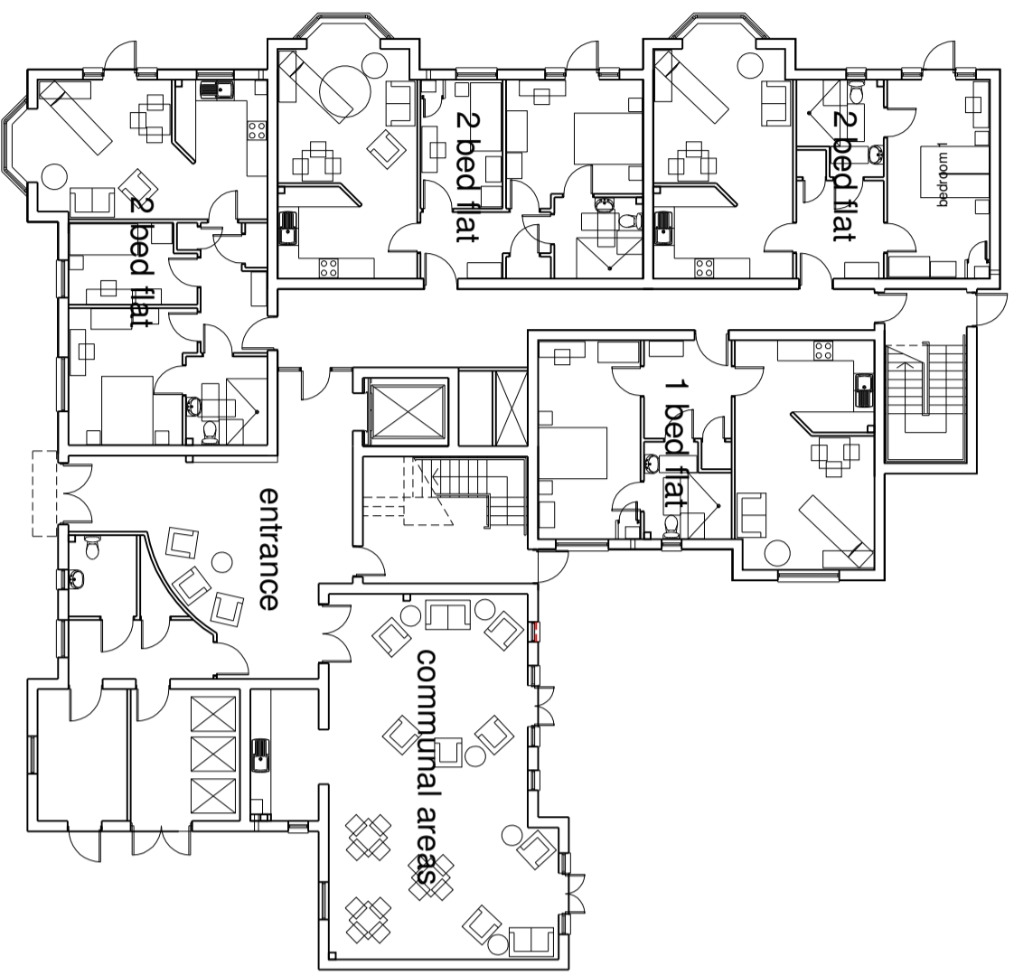
typical ground floor plan of flats for elderly
